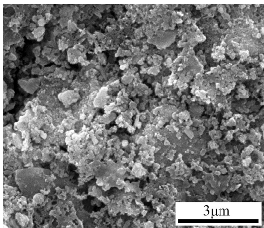
Fig. 5 SEM micrograph of the obtained glass-ceramics
