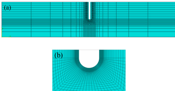
Figure 2. The meshes of the U-shaped edge-notched specimen covered by a CPF: (a) the global and (b) local meshes.
