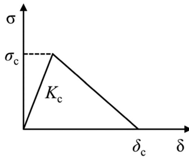
Figure 3. Triangular traction-separation law used in the analysis.
