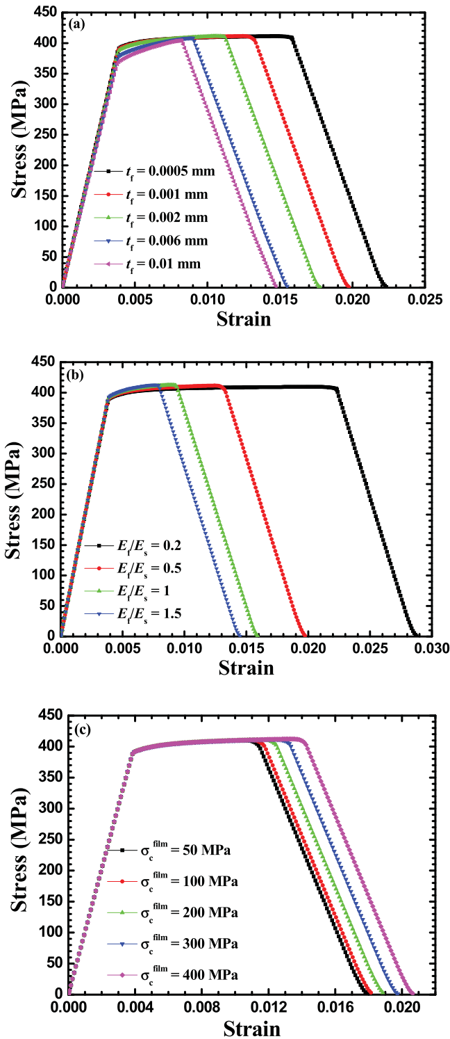
Figure 5. Stress-strain curves obtained from the cohesive zone modelling of the flat specimen with and without CPF with: (a) various CPF thickness and E_f/E_s = 0.5 , and \sigma_c^{\text{CPF}} = 300 MPa; (b) various CPF Young's moduli with t_f = 0.001 mm and \sigma_c^{\text{CPF}} = 300 MPa; (c) various CPF fracture strengths with t_f = 0.001 mm and E_f/E_s = 0.5 .
