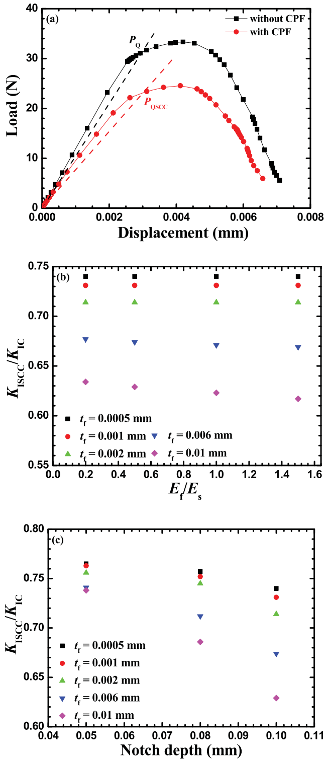
Figure 7. (a) P_Q and P_{QSCC} in the load-displacement curve of the U-shaped edge-notched specimen, and the variation of the normalised threshold stress intensity factor ( K_{ISCC}/K_{IC} ) with: (b) various Young's modulus ratio E_f/E_s and CPF thicknesses for the notch depth of 0.1 mm; (c) various notch depths and CPF thicknesses for the CPF Young's modulus ratio E_f/E_s = 0.5 .
