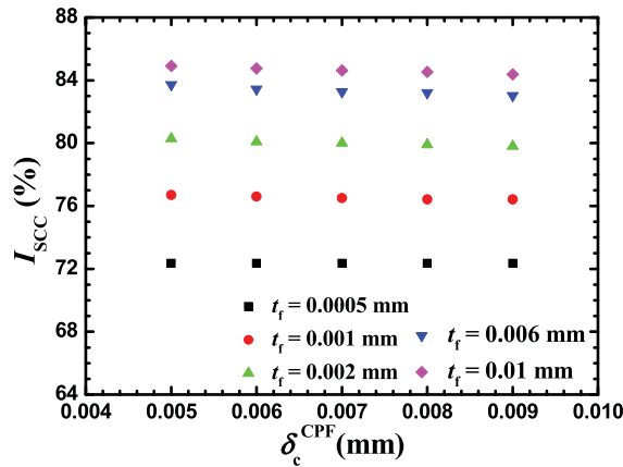
Figure 4. Effect of the critical opening displacement of CPF, \delta_c^{CPF} , on the calculated SCC susceptibility based on the cohesive zone modelling with various CPF thickness and E_f/E_s = 0.5 , and \sigma_c^{CPF} = 300 MPa.
