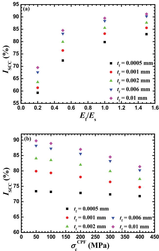
Figure 6. Calculated SCC susceptibility based on the cohesive zone modelling with: (a) various CPF thickness and Young's modulus ratio E_f/E_s for the CPF with \sigma_c^{CPF} = 300 MPa, and (b) various CPF fracture strengths of the CPF with Young's modulus ratio E_f/E_s = 0.5 .
